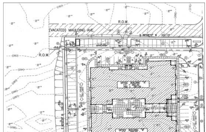
Prototype grading plan for Freeway Office Park , located on Dean Martin Drive.
